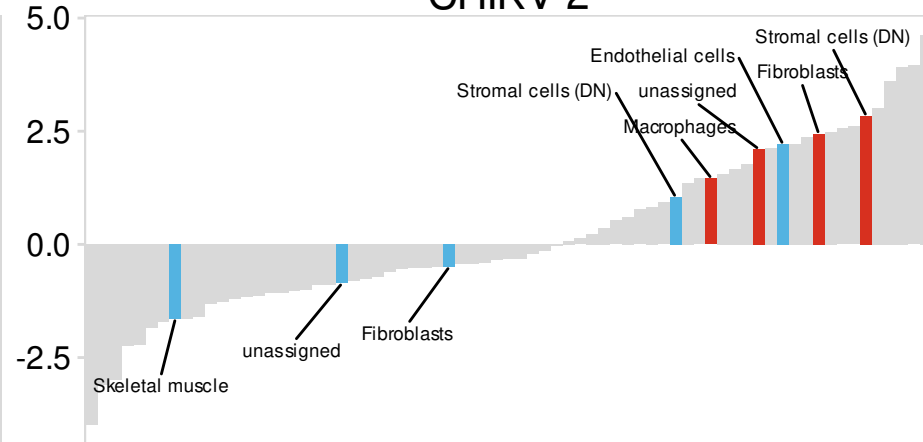
CHIKV-2
